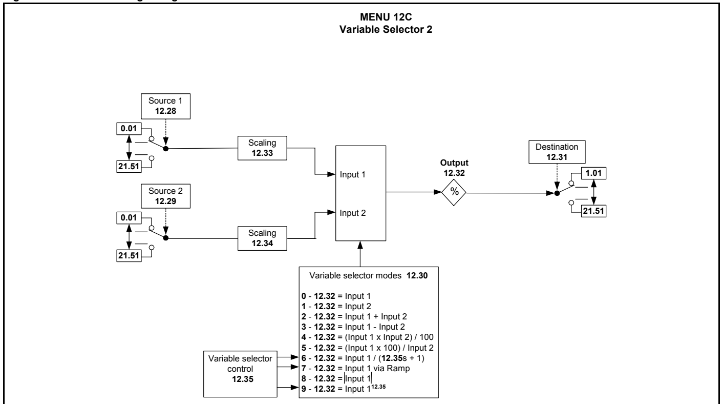
Figure 9-38 Menu 12C logic diagram
