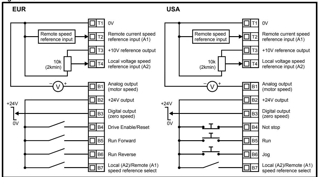
Figure 9-26 Pr 11.27 = AI.AV
