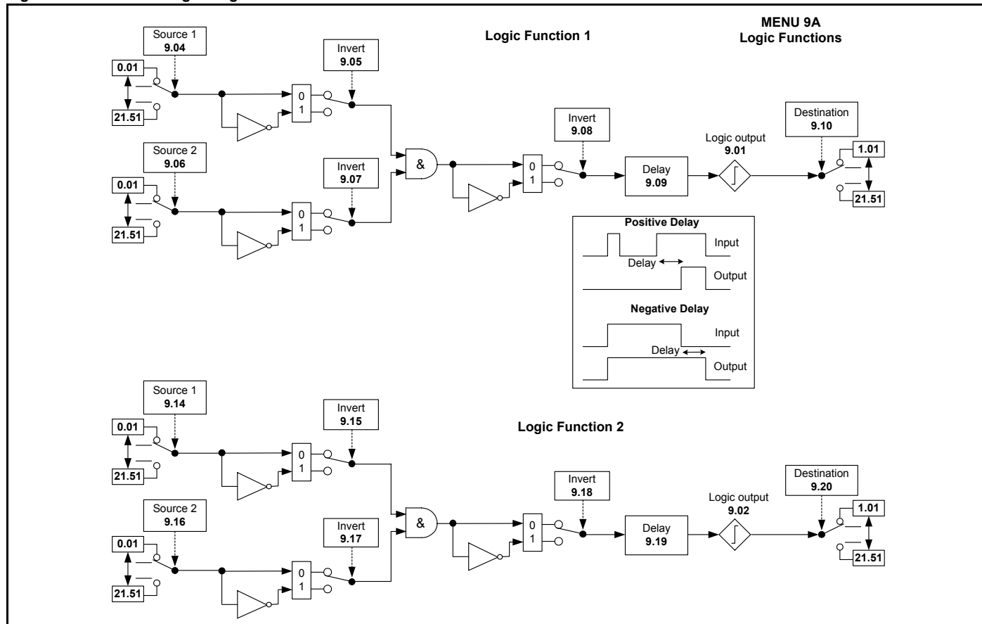
Figure 9-23 Menu 9A logic diagram
