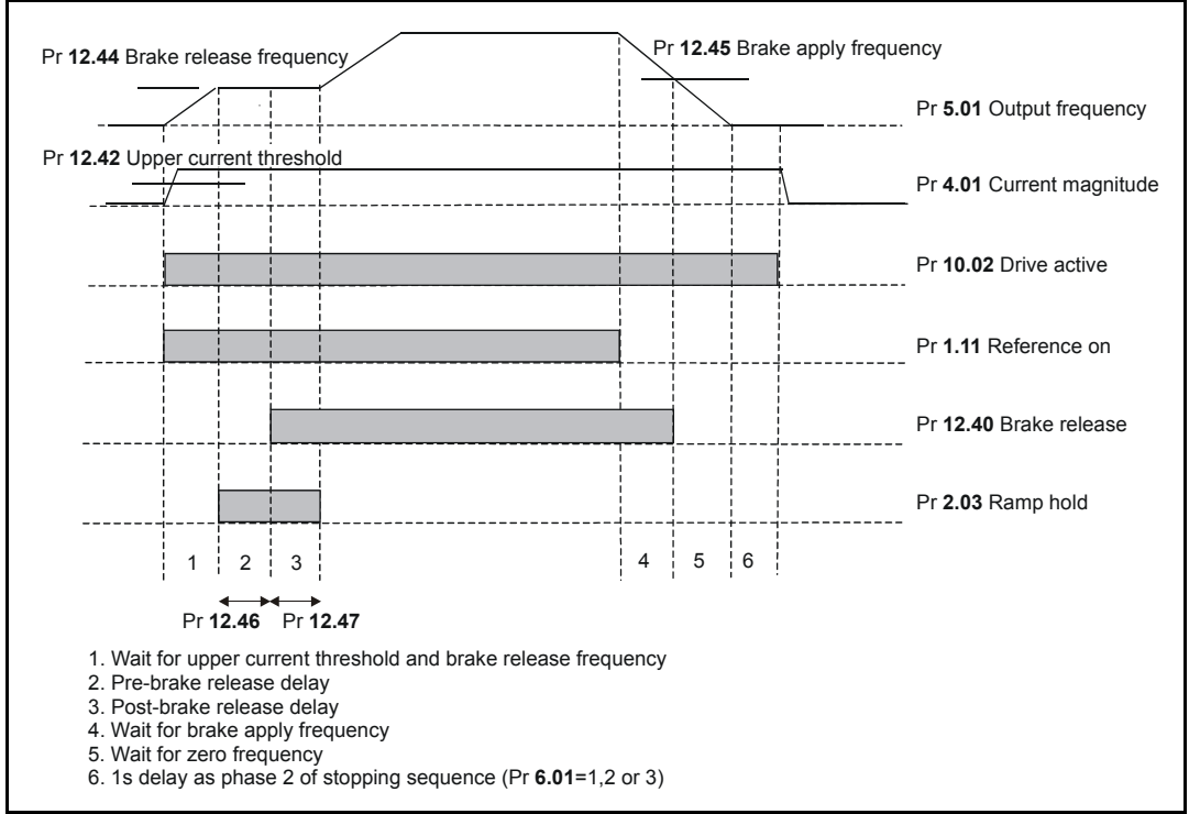
Figure 9-41 Brake sequence
