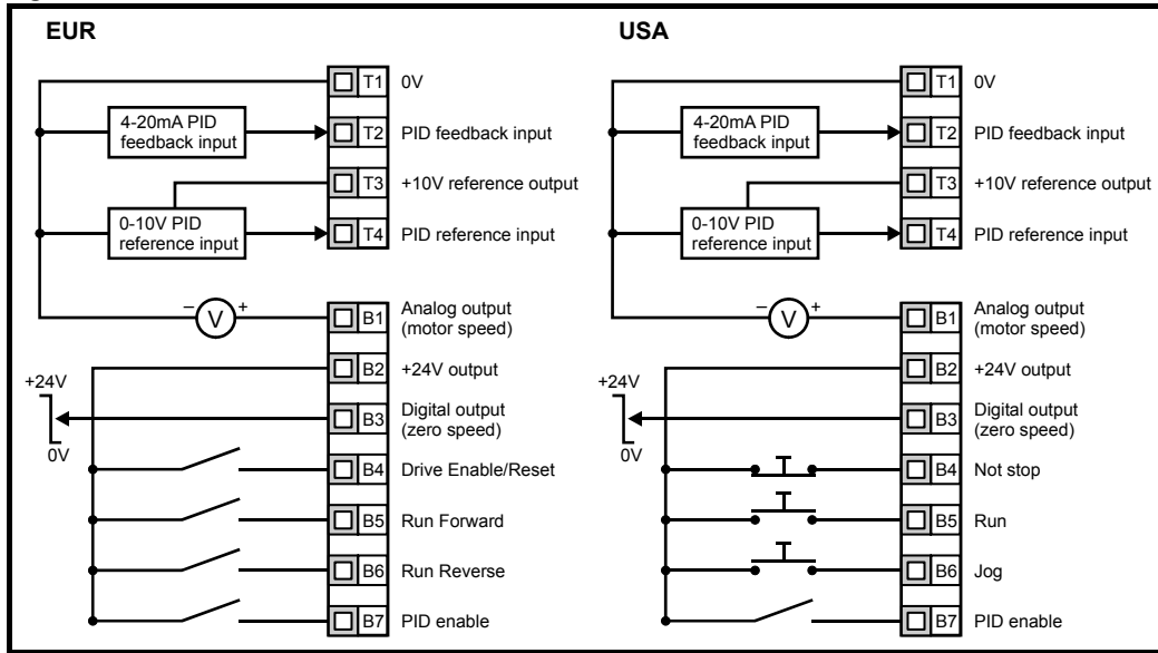
Figure 9-33 Pr 11.27 = Pid
