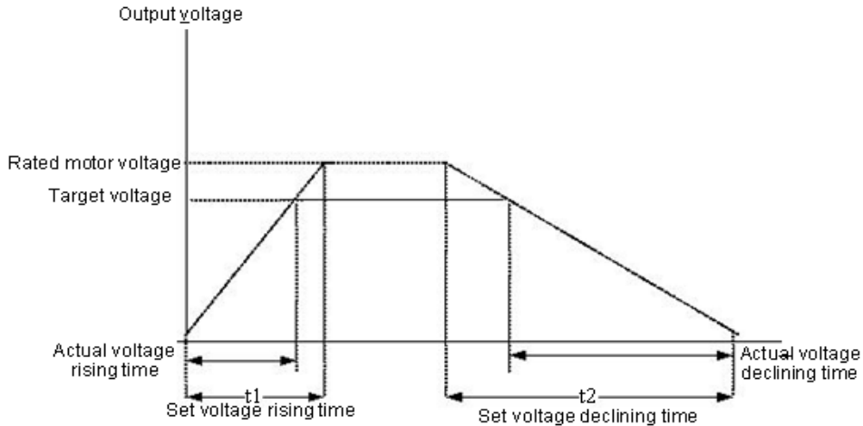
Figure 4-7 Voltage of V/F separation
