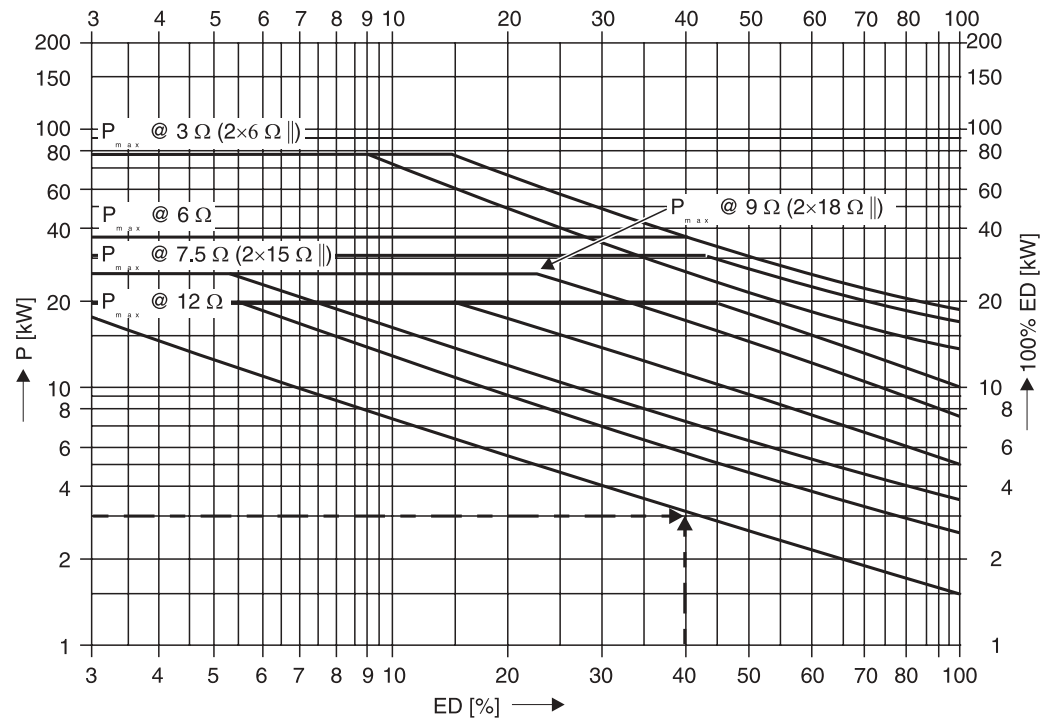
Figure 49: Grid resistor 230 V
