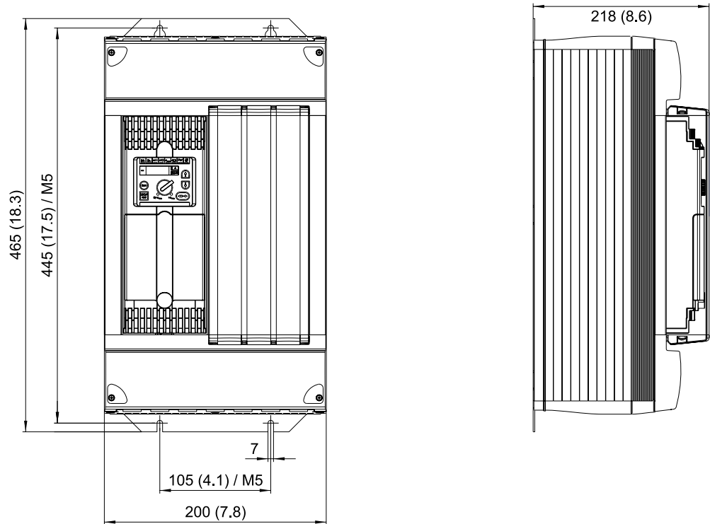
Figure 17: Dimensions, MOVITRAC® 07 size 3
