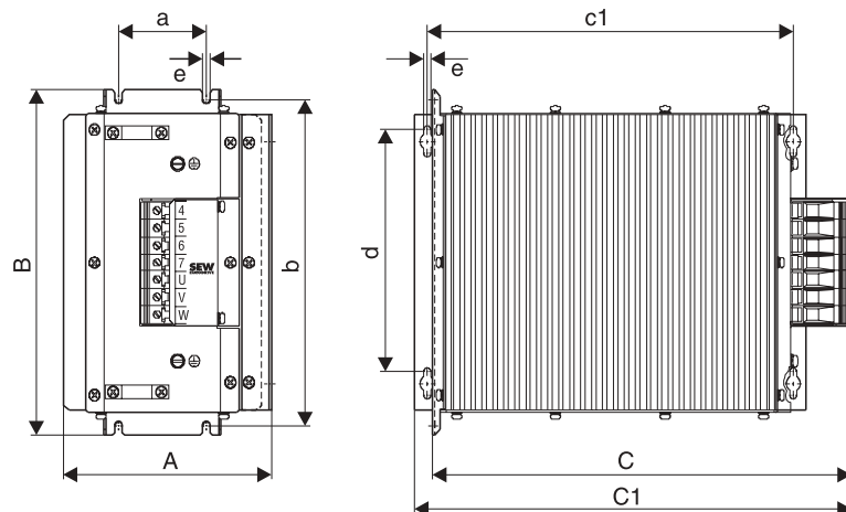
Figure 41: Dimensions HF...-403
