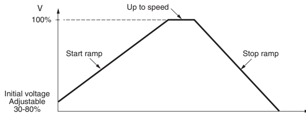
Voltage start and stop ramps, initial voltage, and up to speed
